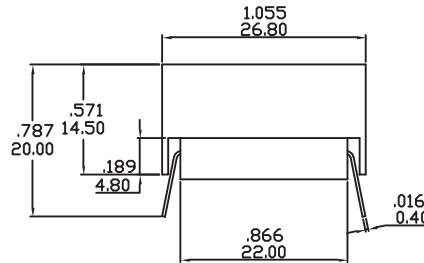
6A 250VAC \phi 5.20x20mm
