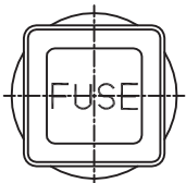
10A 250VAC \phi 6.40x30mm
